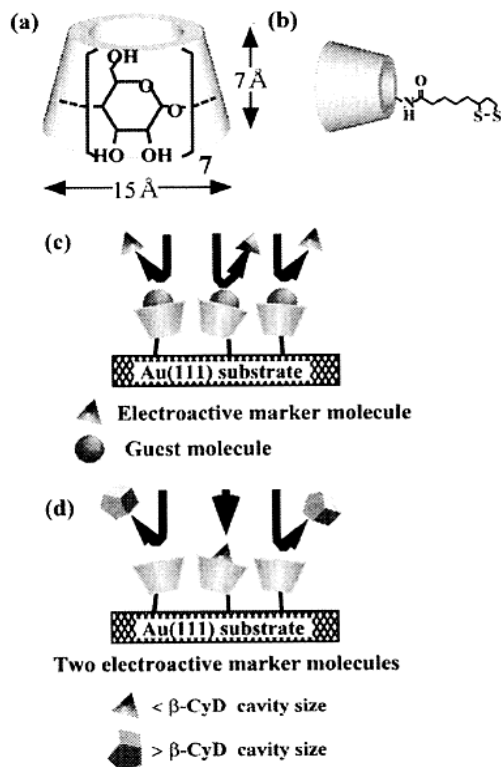
Fig. 1 Schematic structures of (a) \beta -cyclodextrin (b-CyD), (b) \beta -CyD modified with lipoyamide residue (LP- \beta -CyD), and molecular recognition mechanism by LP- \beta -CyD monolayer with (c) and without (d) guest compounds.
