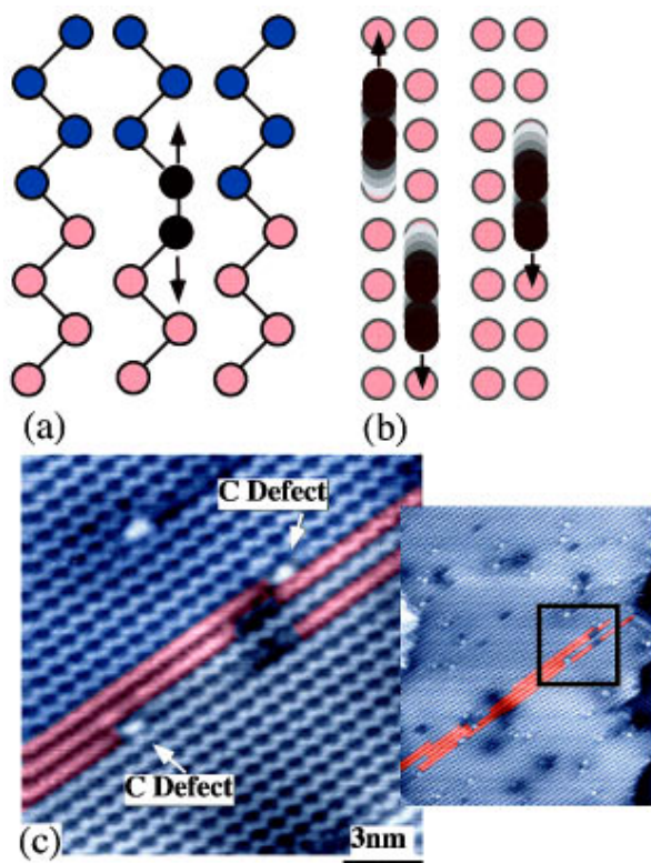
FIG. 2. (a) Stick and ball model showing the down (up) atoms of the buckled dimers. Red and blue represent the c(4 \times 2) and p(2 \times 2) phases, respectively. The schematic structure of the C defect and P defects is represented by the black atoms. (b) Schematic showing many P defects migrating along the dimer rows resulting in an apparent symmetric configuration of dimers observed by STM. (c) The STM image on the right shows a wider region of the STM image on the left (region surrounded by a box). Tunneling conditions: 0.6 V and 1 nA.
