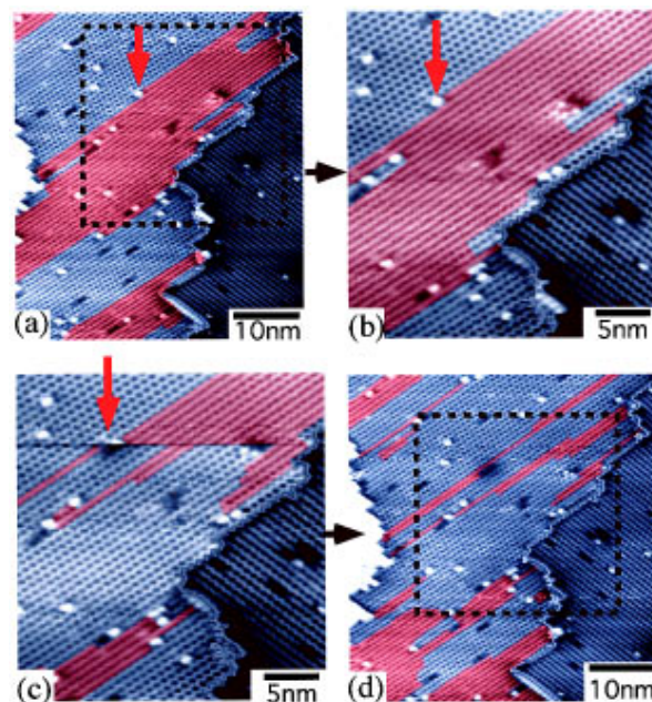
FIG. 3. Another example of perturbation. (a) A large scale STM image showing an overview of a large symmetric region (red). (b) A closeup showing the boundary of the symmetric and buckled dimer domains. (c) The C defect located at the boundary indicated by the red arrows was perturbed. (d) Final configuration after perturbation. Tunneling conditions: 0.6 V and 1 nA.
