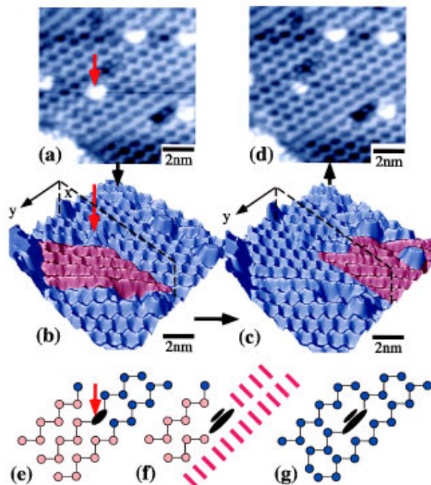
FIG. 1. Four STM images showing the dynamical response of the surface to a perturbation. The red regions show the symmetric dimer domains induced by the perturbation. Tunneling conditions: 0.6 V and 1 nA. The schematics show the stick and ball atomic structure of the initial, excited, and final states.
