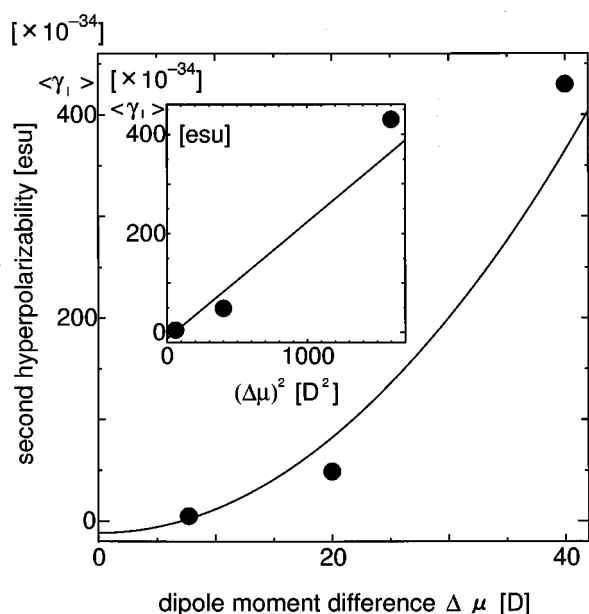
FIG. 2. Dependence of second hyperpolarizability ( \langle \gamma_i \rangle ) on permanent electric dipole-moment difference between excited and ground states ( \Delta \mu ) for different ICT molecules. Inset, (\Delta \mu)^2 plot of \langle \gamma_i \rangle .
