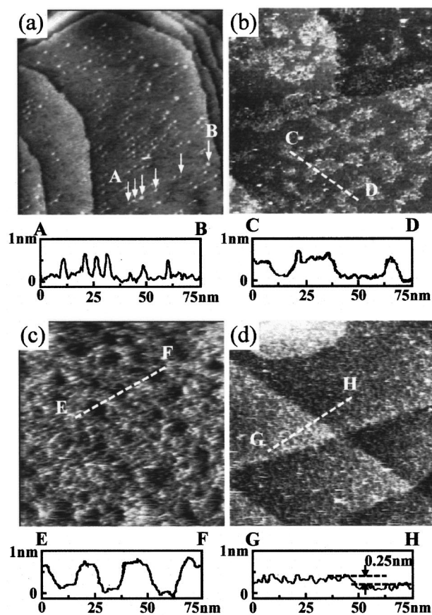
FIG. 2. STM images of LP- \beta -CyD on Au(111) ( 150 \text{ nm} \times 150 \text{ nm} ) formed by different immersion times, (a) 3 s ( V_s = 1.0 \text{ V} , I_t = 0.2 \text{ nA} ), (b) 6 s ( V_s = 2.0 \text{ V} , I_t = 0.3 \text{ nA} ), (c) 60 s ( V_s = 1.0 \text{ V} , I_t = 0.2 \text{ nA} ), and (d) 10 min ( V_s = 2.0 \text{ V} , I_t = 0.2 \text{ nA} ), respectively.
