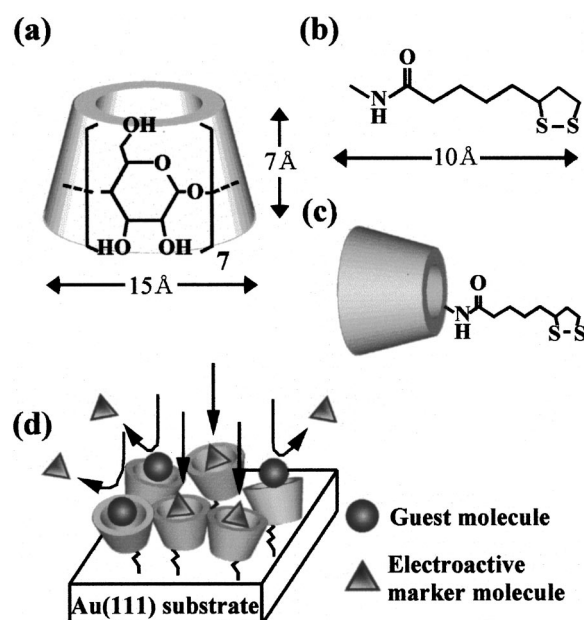
FIG. 1. Schematic structures of (a) \beta -CyD, (b) LP, (c) \beta -CyD modified with LP, and (d) molecular recognition by LP- \beta -CyD monolayer.
