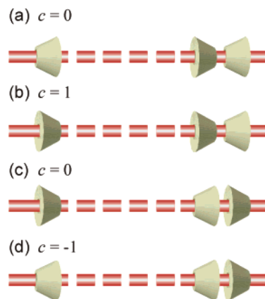
Figure 10. Four conformations of the CyDs in a molecular necklace and the corresponding values of c appearing in eq 6: (a) and (c) CyD molecules with both ends having the same orientation ( c = 0 ). (b) CyD molecules with both ends having the tail-to-tail conformation ( c = 1 ). (d) CyD molecules with both ends having the head-to-head conformation ( c = -1 ).
