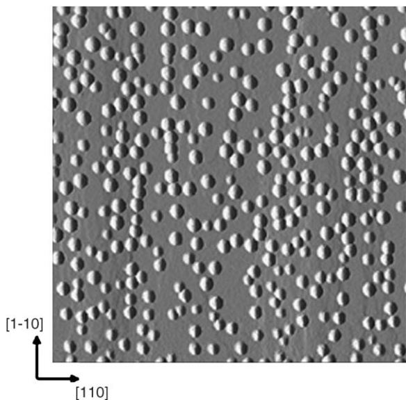
Fig. 1. AFM image of typical InAs QD structure grown on GaAs (001) substrate. Scan size is 1 \mu\text{m} \times 1 \mu\text{m} .
