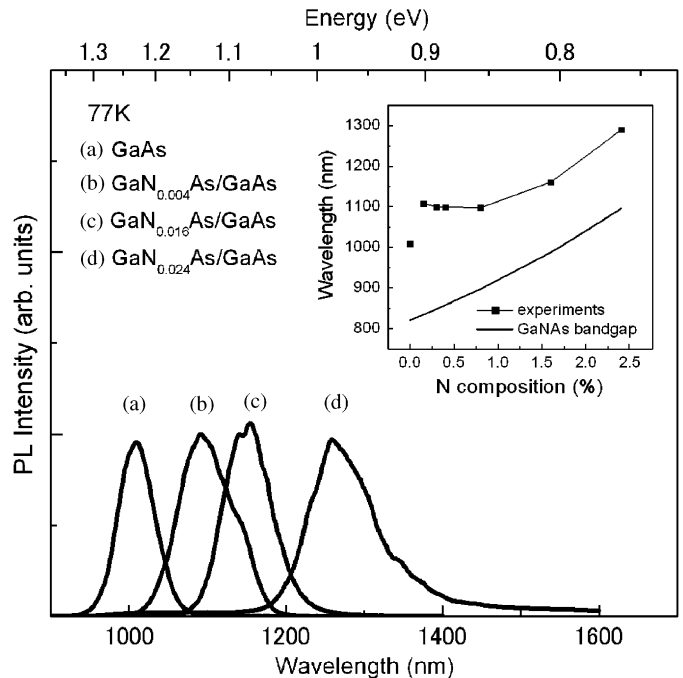
Fig. 2. PL spectra at 77 K from InAs QDs embedded in \text{GaN}_x\text{As}_{1-x} SCLs with varying N composition. Inset shows center peak wavelength as a function of N composition.
