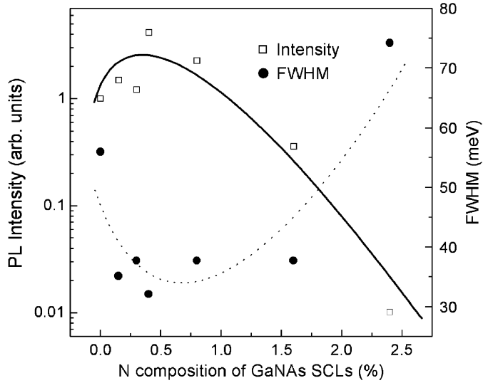
Fig. 3. Integral PL intensity (open square) and full width at half-maximum (FWHM) (circle) as a function of N composition of GaNAs SCL.
