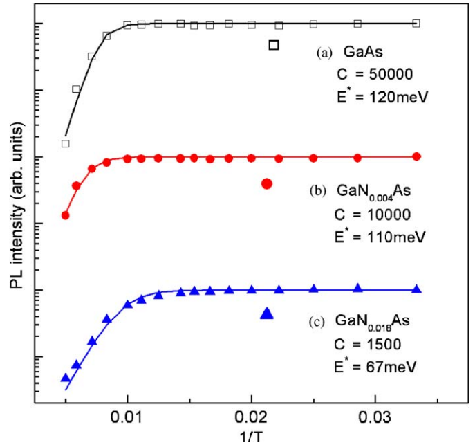
Fig. 4. Temperature dependence of PL intensity from InAs QDs covered by (a) GaAs, (b) \text{GaN}_{0.004}\text{As} , and (c) \text{GaN}_{0.016}\text{As} , respectively.
