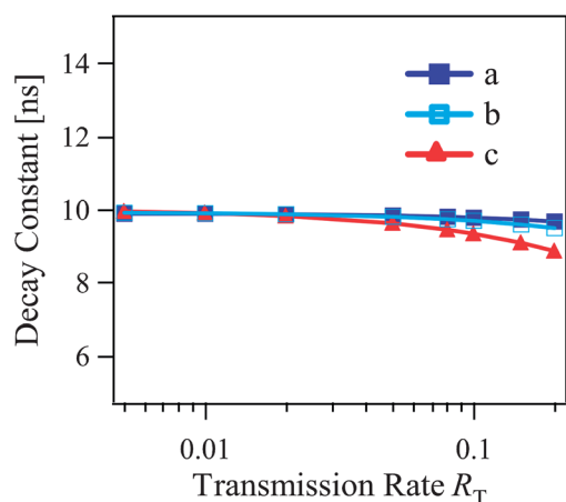
Fig. 5 Simulation results for analysis of hole dynamics via the in-gap state shown in Fig. 1(e): decay constant \tau_g as a function of R_T for three different laser intensities ((a) 5 \times 10^{12} , (b) 1 \times 10^{13} , (c) 3 \times 10^{13} \text{ cm}^{-3} ). The parameters used were V_s = 1 \text{ V} , I_0 = 50 \text{ pA} , N_{\text{ex}} = 2 \times 10^{14} \text{ cm}^{-3} , n_0 = 10^{18} \text{ cm}^{-3} , \tau_d = 1 \text{ } \mu\text{s} and \tau_g = 10 \text{ ns} .
