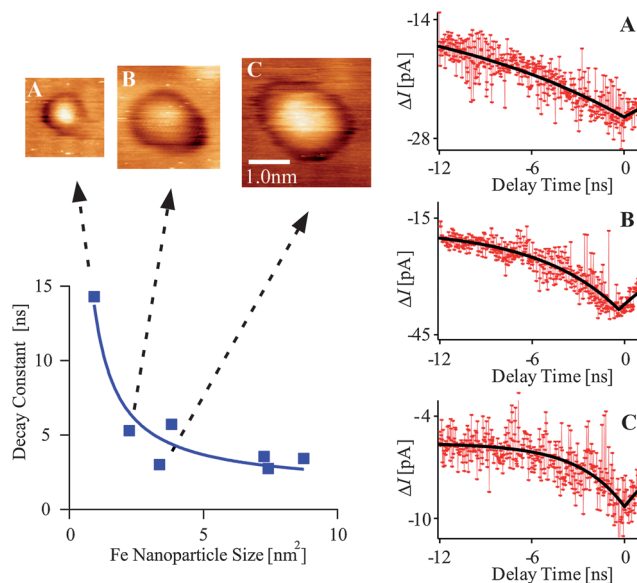
Fig. 6 Decay constant of the density of photoinduced holes transiently trapped at the surface as a function of the Fe nanoparticle size on a GaAs(110) surface. Three spectra with a single exponential fitting curve, which were obtained above the Fe nanoparticles shown by STM images, are shown together (the size of the Fe nanoparticle in image A corresponds to a single Fe atom).
