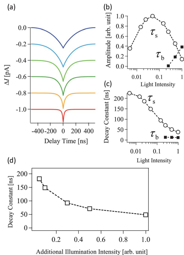
Fig. 3 Results of simulations carried out for comparison with experimental results shown in Fig. 2. Simulations shown in (a) to (c) were carried out at eight points corresponding to those in (a) to (c) (six of them are shown in (a)). The dependence of the additional illumination intensity of the surface side decay shown in (d) was calculated for five intensities and compared with the experimental results shown in Fig. 2(d). The parameters used were V_s = 1 V, I_0 = 50 pA, N_{\text{ex}} = 2 \times 10^{14} cm ^{-3} , n_0 = 10^{18} cm ^{-3} , \tau_d = 1 \mu s, n'_0 = 2 \times 10^{15} cm ^{-3} , \tau_b = 10 ns and A = 10^5 .
