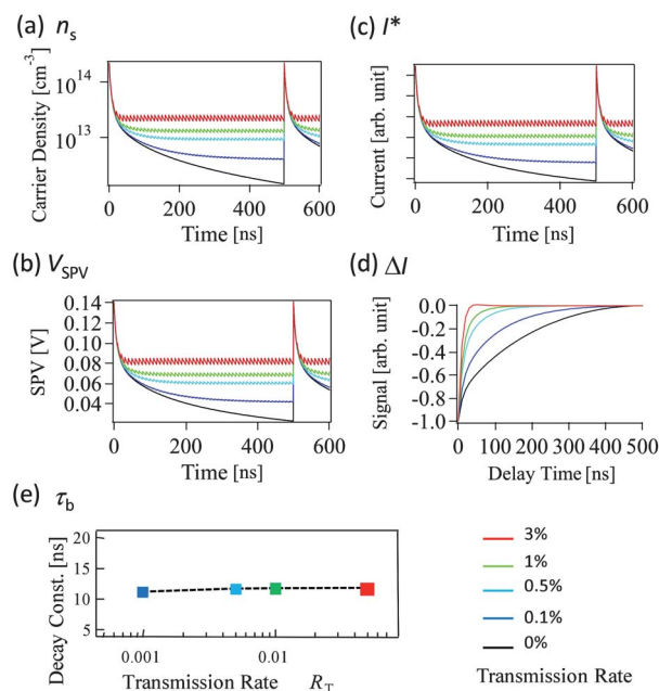
Fig. 4 Simulation results of five transmission rates R_T for four processes in OPP-STM measurement: (a) n_s(t) , (b) \text{SPV}(t) , (c) I^*(t) , and (d) \Delta I(t) . (e) Transmission rate dependence of \tau_b . The parameters used were V_s = 1 V, I_0 = 50 pA, N_{\text{ex}} = 2 \times 10^{14} cm ^{-3} , n_0 = 10^{18} cm ^{-3} , \tau_d = 1 \mu s, n'_0 = 2 \times 10^{15} cm ^{-3} , \tau_b = 10 ns and A = 10^5 .
