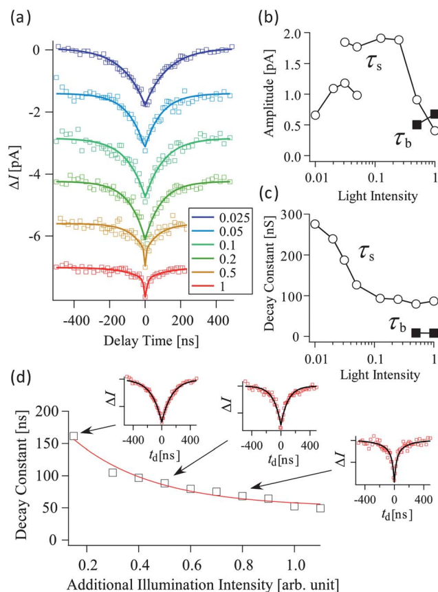
Fig. 2 (a) Laser-intensity dependence of OPP-STM spectra obtained for the GaAs(110) sample (set point: V_s = 1 \text{ V} , I_t = 100 \text{ pA} ). The laser intensity was normalized with the maximum value of 4 mW. Amplitudes (b) and decay constants (c) were obtained by the exponential fitting of the spectra in (a) (typical six spectra are shown in (a)). (d) Decay constant as a function of additional laser intensity.
