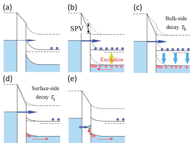
Fig. 1 Schematic illustrations of 1D band structures in OPP-STM measurement of the bare surface ((a) to (d)) and the surface with the in-gap state (e).
