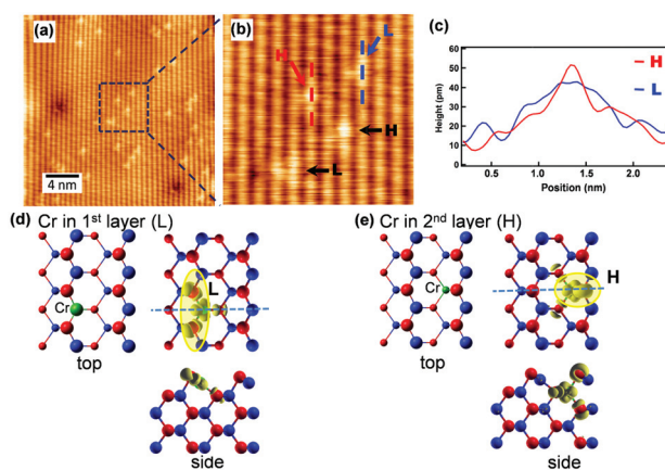
Fig. 2 STM observation of Cr atoms on a (Zn,Cr)Te surface. (a) High resolution STM image of Cr dopant atoms on a (Zn,Cr)Te(110) surface ( V_s = -2.0 V, I = 10 pA). (b) Magnified image of the area indicated by the dotted square in (a). H and L indicate the two types of images with two different heights. (c) Cross sections obtained along the two dashed lines in (b). (d) and (e) Results of the DFT calculations for the Cr atoms located in the first and second (110) atomic layers, respectively. Spatial distributions are the LDOS integrated over E_F - 0.1 eV < E < E_F ( E_F : Fermi energy). The side-view images below represent cross-sectional drawings along the dashed lines in the respective top-view images.
