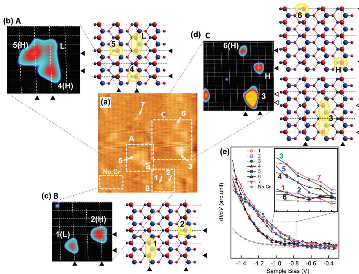
Fig. 3 STM/STS analyses of Cr–Cr interaction. (a) STM image of the (Zn,Cr)Te area ( V_s = -2.0 V, I = 20 pA). (b), (c) and (d) Left: magnified images of the square areas indicated by A, B and C in (a), respectively. Low-pass filtering was carried out to enhance the local electronic structures. Right: schematic structures of the atomic configurations of the STM images on the left. (e) dI/dV - V spectra measured above the Cr atoms labeled #1 to #7 and on the area of ZnTe without Cr in the bottom-left square shown in (a). The inset is a magnification of the dI/dV - V curves in the square region.
