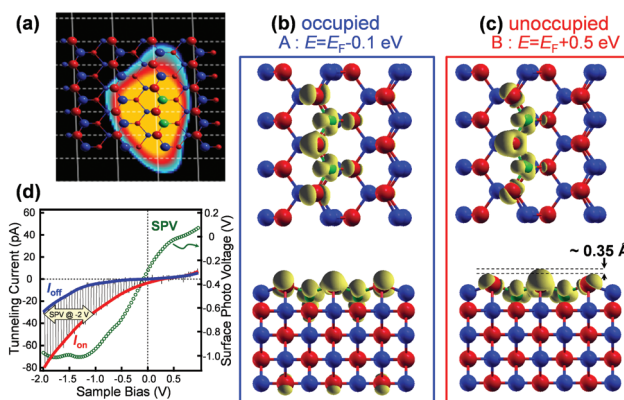
Fig. 4 STM image and DFT calculations for the structure labeled 3 in Fig. 3. (a) Magnification of the low-pass filtered image of label 3 shown in Fig. 3(d) and schematic of its structural model. Results of DFT calculations of local density of states (LDOS) integrated over (b) E_F - 0.1 eV < E < E_F and (c) E_F < E < E_F + 0.5 eV. (d) Typical LM-STs spectra obtained on (Zn,Cr)Te measured with a semiconductor laser ( \lambda = 400 nm, light-intensity = 5 mW). For example, the yellow arrow indicates the magnitude of the surface photo voltage at V_s = -2.0 V.
