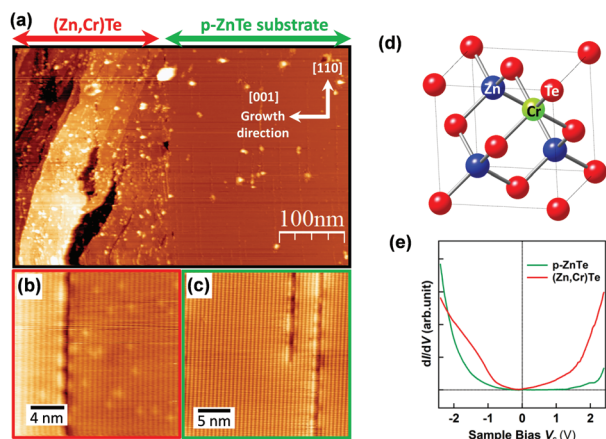
Fig. 1 STM/STS measurements of (Zn,Cr)Te/p-ZnTe. (a) Cross-sectional STM topographic image of the (Zn,Cr)Te/p-ZnTe multilayered structure ( V_s = +5.0 V, I = 20 pA). (b) and (c) Magnified STM images of the (Zn,Cr)Te layer ( V_s = -2.0 V, I = 40 pA) and the p-ZnTe substrate ( V_s = -1.5 V, I = 60 pA), respectively. (d) Schematic view of the (Zn,Cr)Te unit cell including a substitutional Cr atom. (e) dI/dV-V spectra averaged over the (Zn,Cr)Te and ZnTe areas shown in (a).
