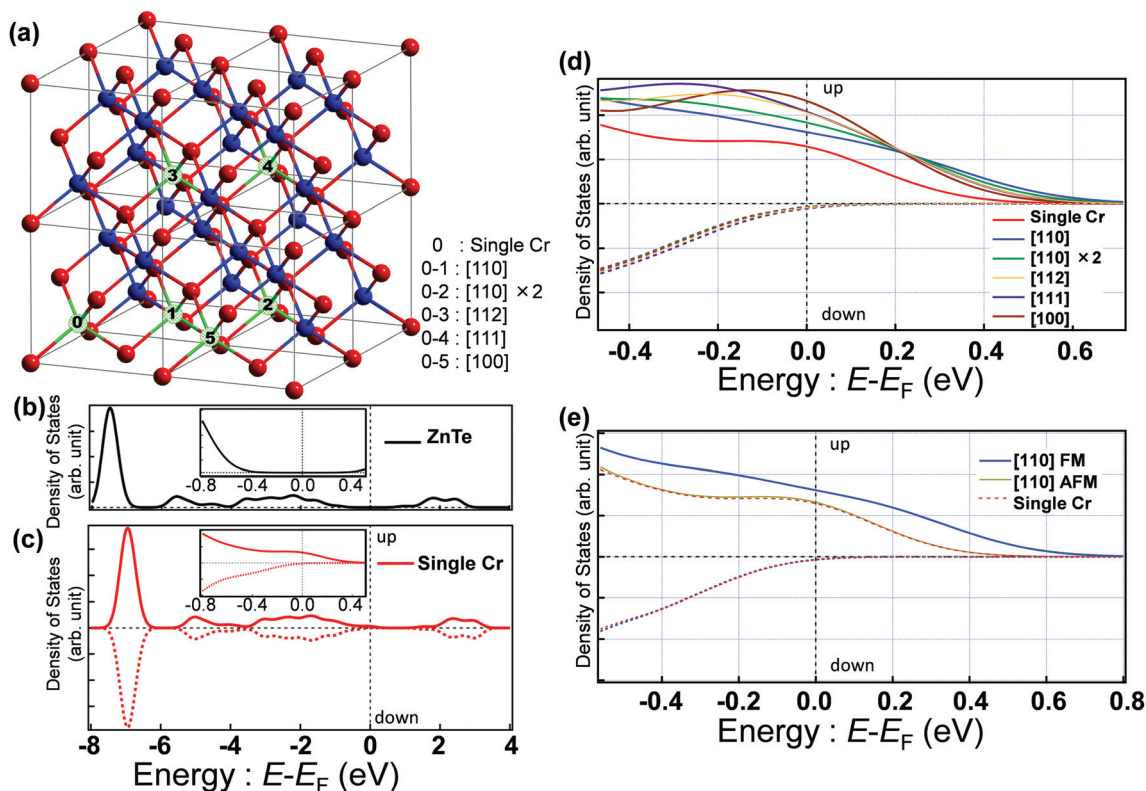
Fig. 5 DFT calculations of DOS for ZnTe and (Zn,Cr)Te structures. (a) Schematic structure of the 2 \times 2 \times 2 supercell used for calculations. One (0) Zn or two (0 and one of 1–5) Zn atoms of the 32 Zn sites were replaced by one/two Cr atoms in the calculations. (b) DOS obtained for undoped ZnTe. (c) DOS obtained for the ZnTe doped with a single Cr atom at the site labeled 0. Up and down indicate spin directions. (d) DOS calculated for various Cr–Cr configurations indicated by different colored lines. (e) DOS calculated for the Cr–Cr structures with ferromagnetic and antiferromagnetic spin orientations.
