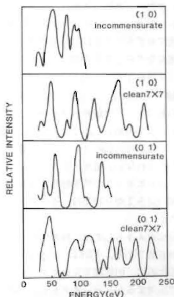
Fig. 5 Comparison between I-V curves from clean Si(111) 7 \times 7 surface and Si(111)-Al incommensurate surface at normal incidence.
